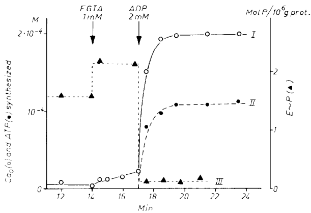
Fig. 1. Labelling of the SR-protein by [ ^{32}\text{P} ] orthophosphate and reversal of the SR calcium pump. Reaction mixture contains (mM) 2 AcP, 7 \text{MgCl}_2 , 20 orthophosphate, 100 glucose, 0.2 \text{CaCl}_2 , 0.02 mg/ml HK and 0.5 mg/ml SR protein (pH 7). The mixture for the measurement of the calcium translocation was labelled with [ ^{45}\text{Ca} ] \text{CaCl}_2 (curve I) and those for the measurement of ATP synthesis and phosphoprotein formation with [ ^{32}\text{P} ] orthophosphate (curve II and III, respectively). During the pre-incubation time (10 min), the vesicles accumulated calcium added in the medium.
